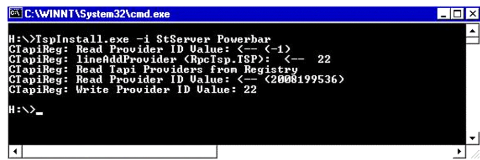
Figure F-2 TSPInstall Command Line
