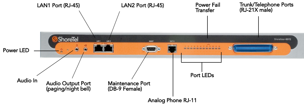
Figure 13-6 The ShoreGear-60/12 Connectors and LEDs
