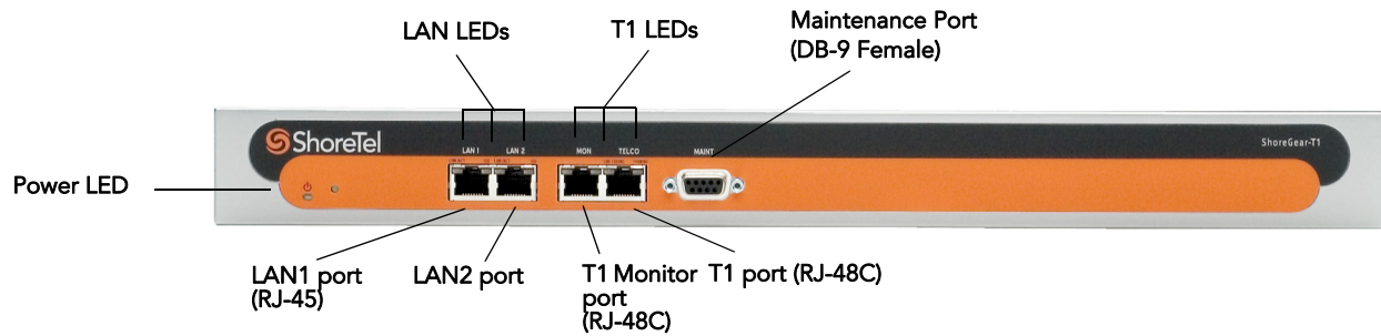
Figure 13-9 ShoreGear-T1 Connectors and LEDs
