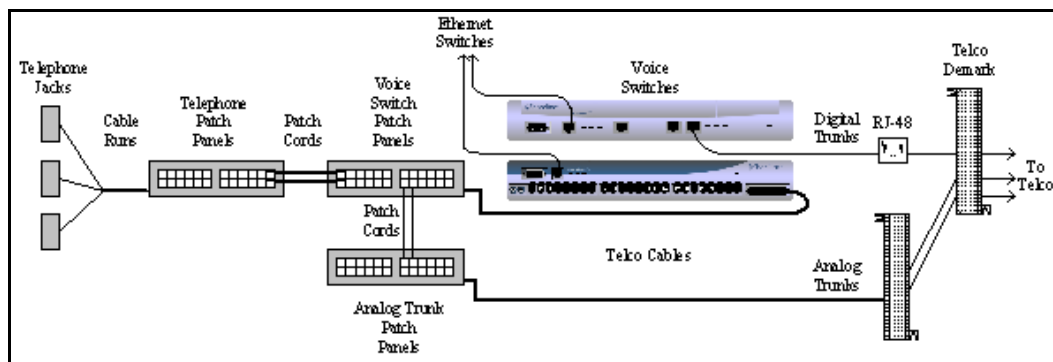
Figure C-5 Cabling Overview
