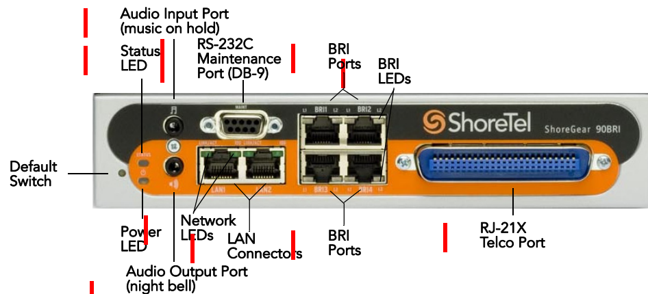
Figure 13-5 ShoreGear 90BRI Connectors and LEDs
