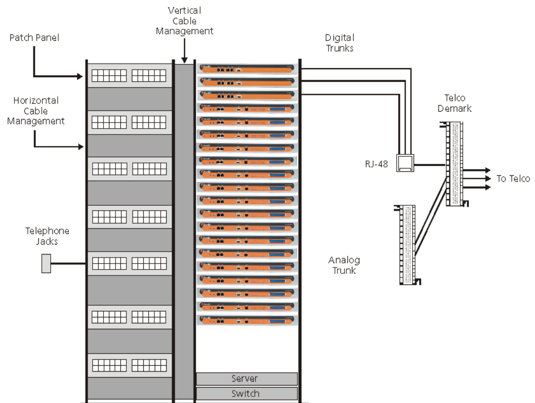
Figure 13-15 Rack Installation
