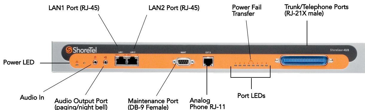
Figure 13-8 ShoreGear-40/8 Connectors and LEDs
