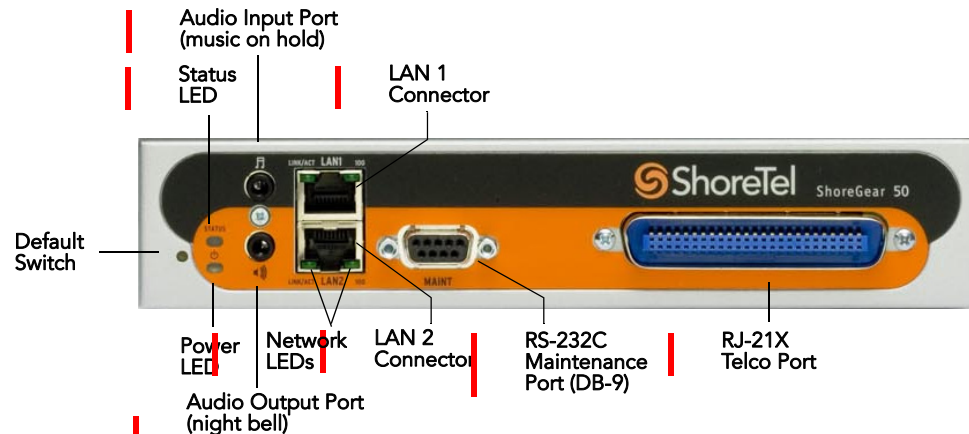
Figure 13-7 ShoreGear 50 Connectors and LEDs
