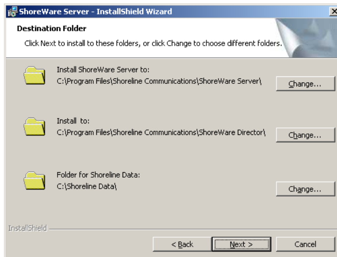
Figure 17-7 Choose Destination for ShoreWare Server and Data Files
