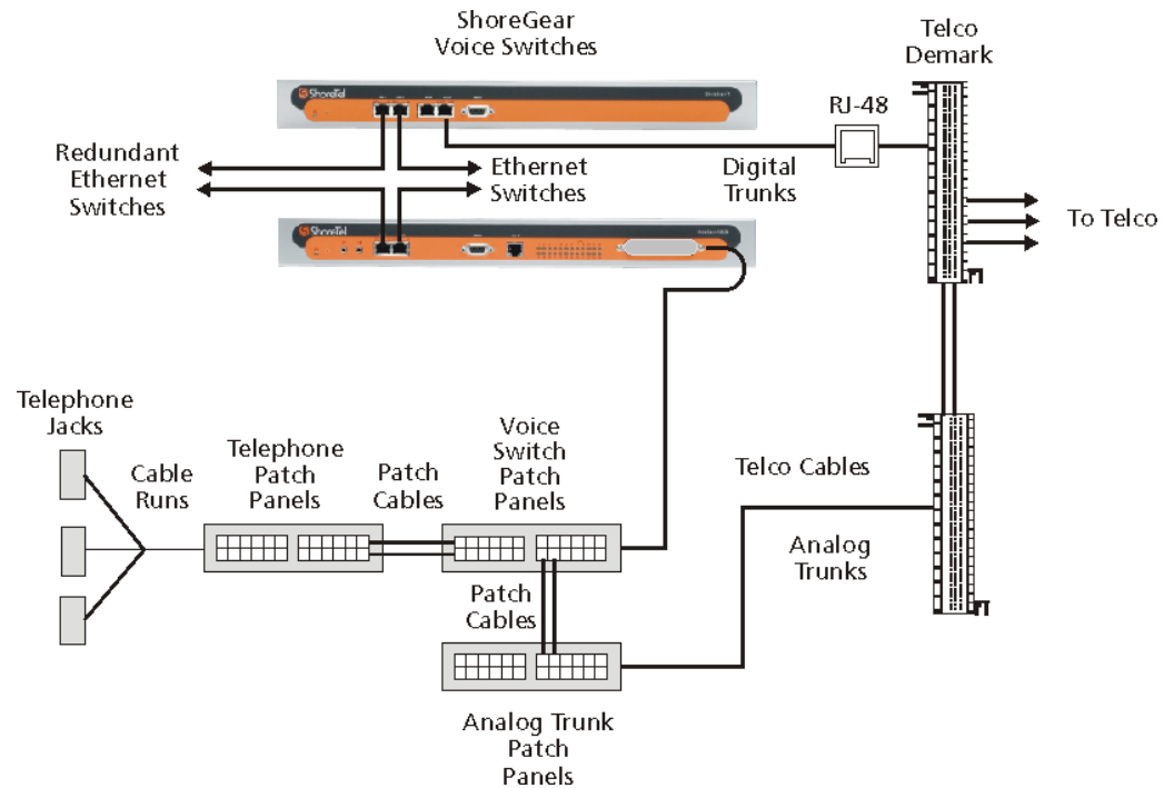
Figure 13-14 Cabling Overview
