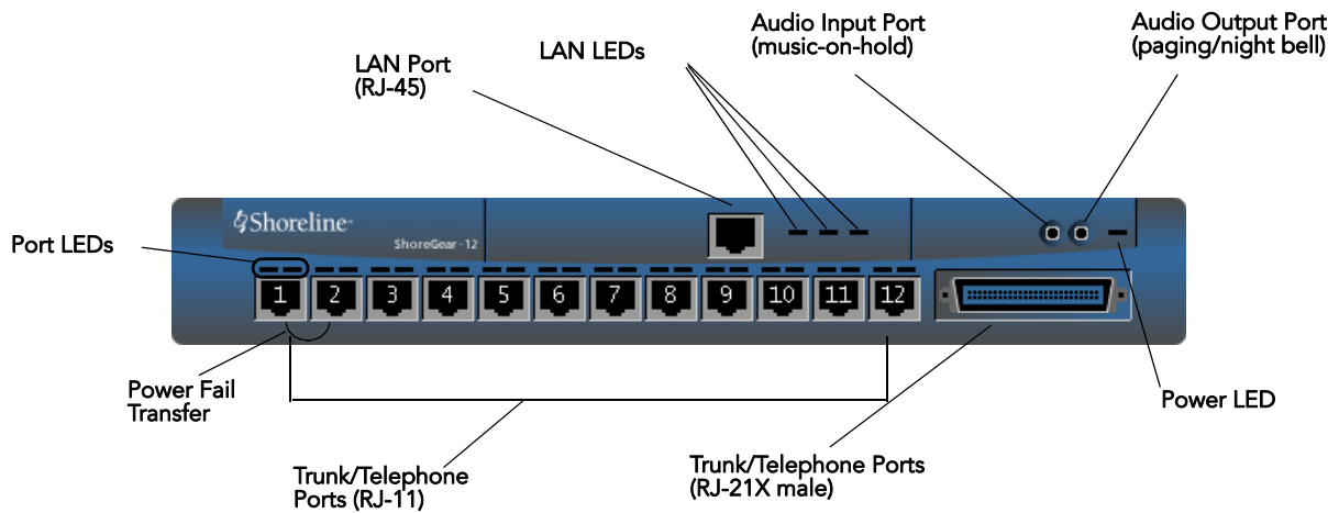
Figure C-2 ShoreGear-12 Connectors and LEDs
