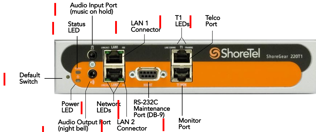
Figure 13-11 ShoreGear 220T1 Connectors and LEDs
