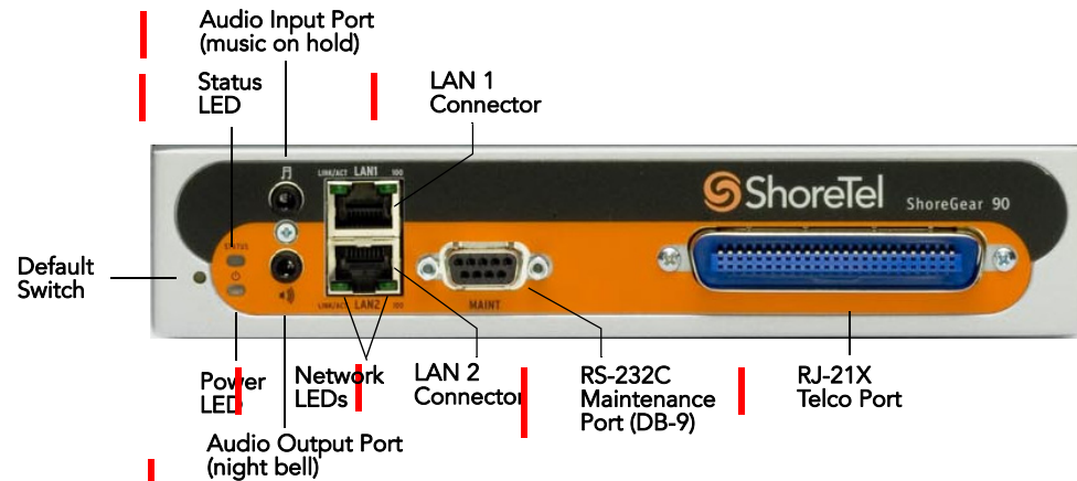
Figure 13-4 ShoreGear 90 Connectors and LEDs
