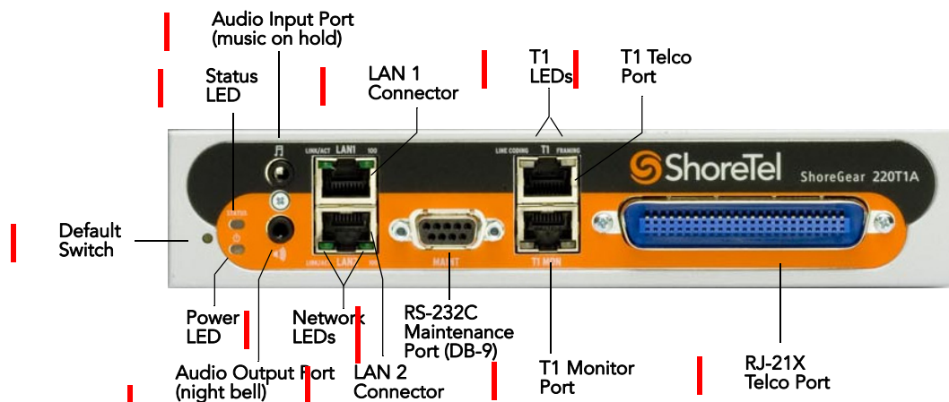
Figure 13-13 ShoreGear 220T1A Connectors and LEDs
