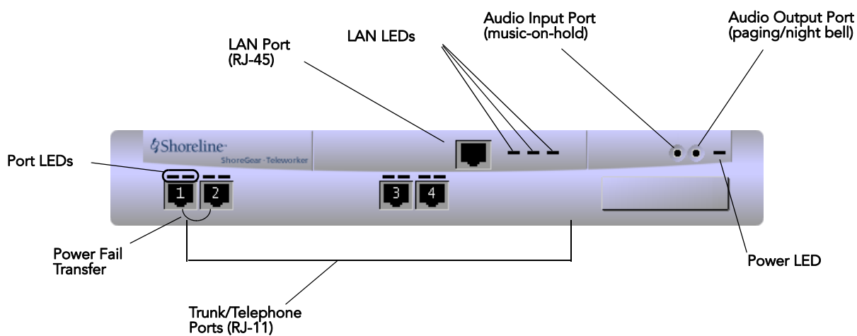
Figure C-3 ShoreGear-Teleworker Connectors and LEDs
