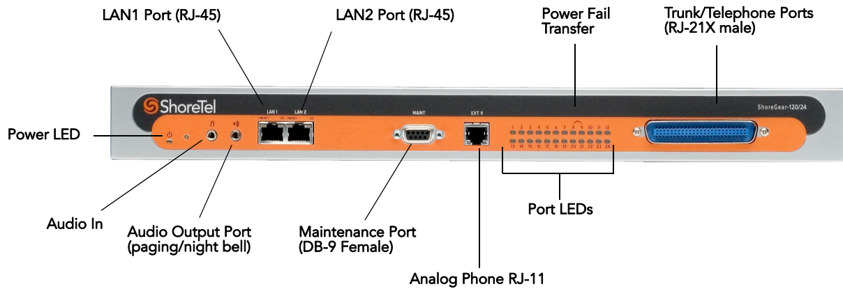
Figure 13-3 ShoreGear-120/24 Connectors and LEDs
