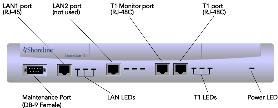
Figure C-4 ShoreGear-T1 Connectors and LEDs
