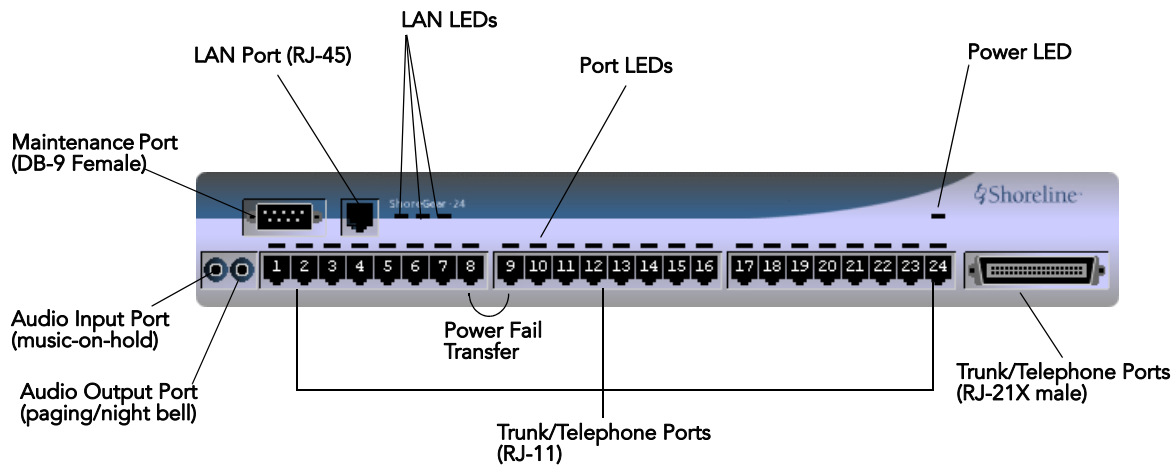
Figure C-1 ShoreGear-24 Connectors and LEDs
