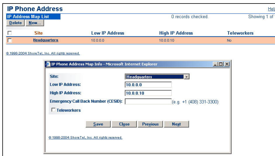
Figure 15-2 IP Address Map List and IP Address Range Edit Pages
