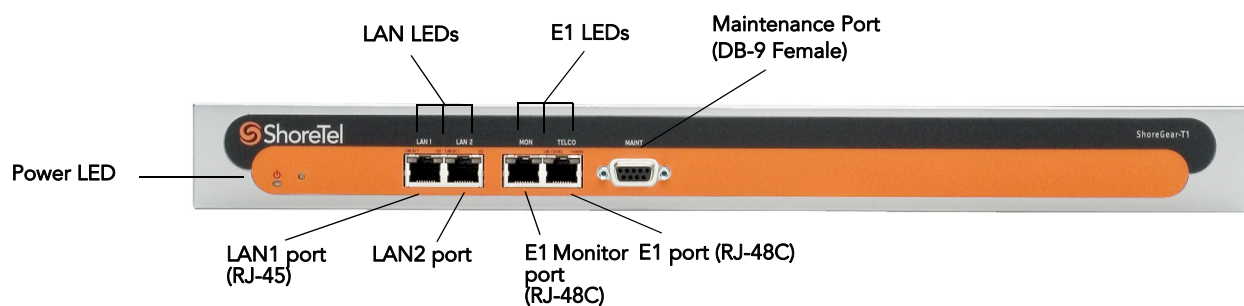
Figure 13-10 ShoreGear-E1 Connectors and LEDs
