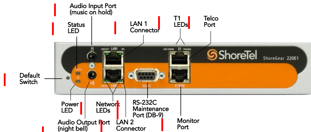
Figure 13-12 ShoreGear 220E1 Connectors and LEDs
