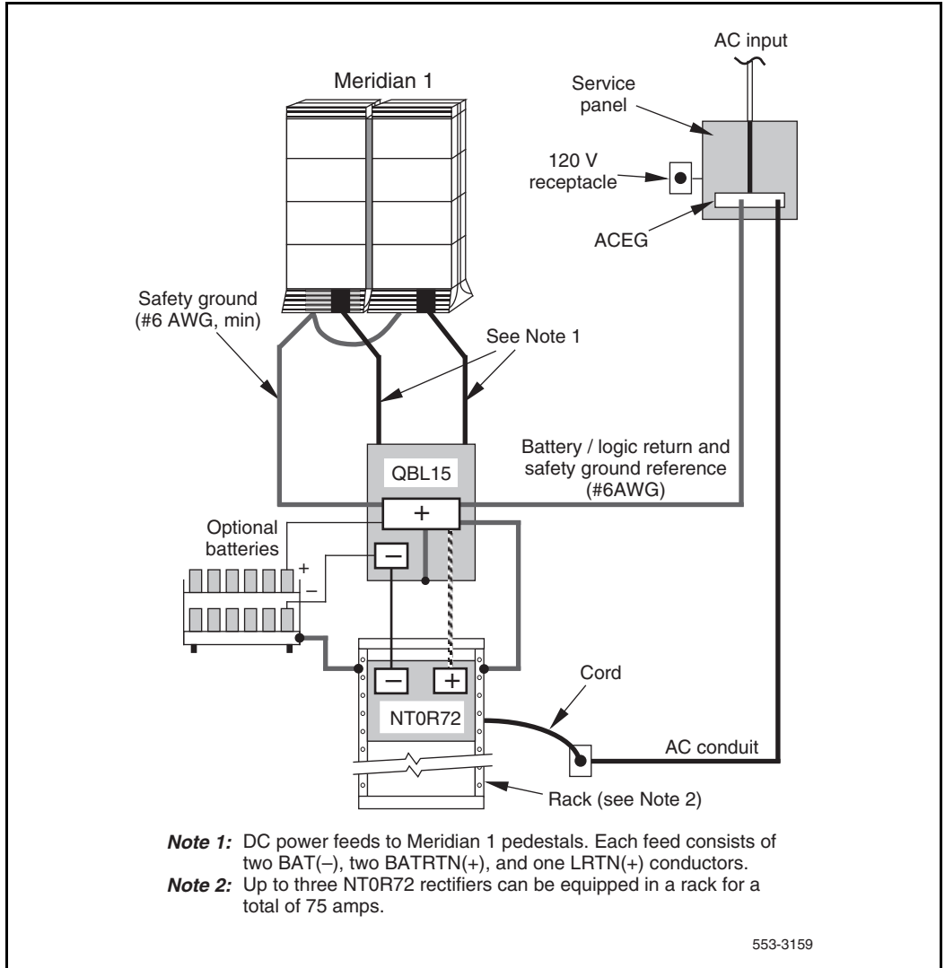
Figure 24 DC power—multiple-column distribution with J2412 Power Plant
