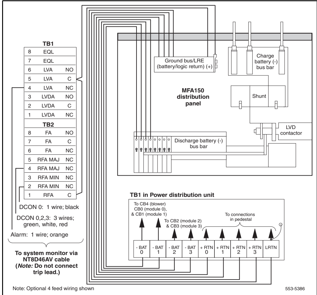
Figure 33 PDU to MFA150 connections
