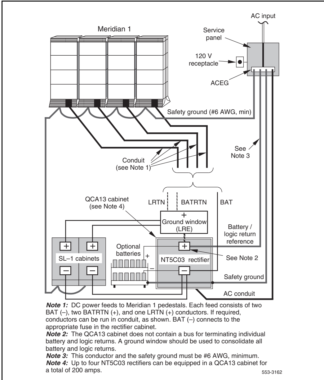
Figure 25 DC power—example of upgraded system distribution
