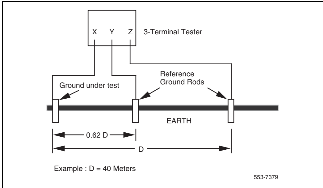
Figure 9 Three terminal testing
