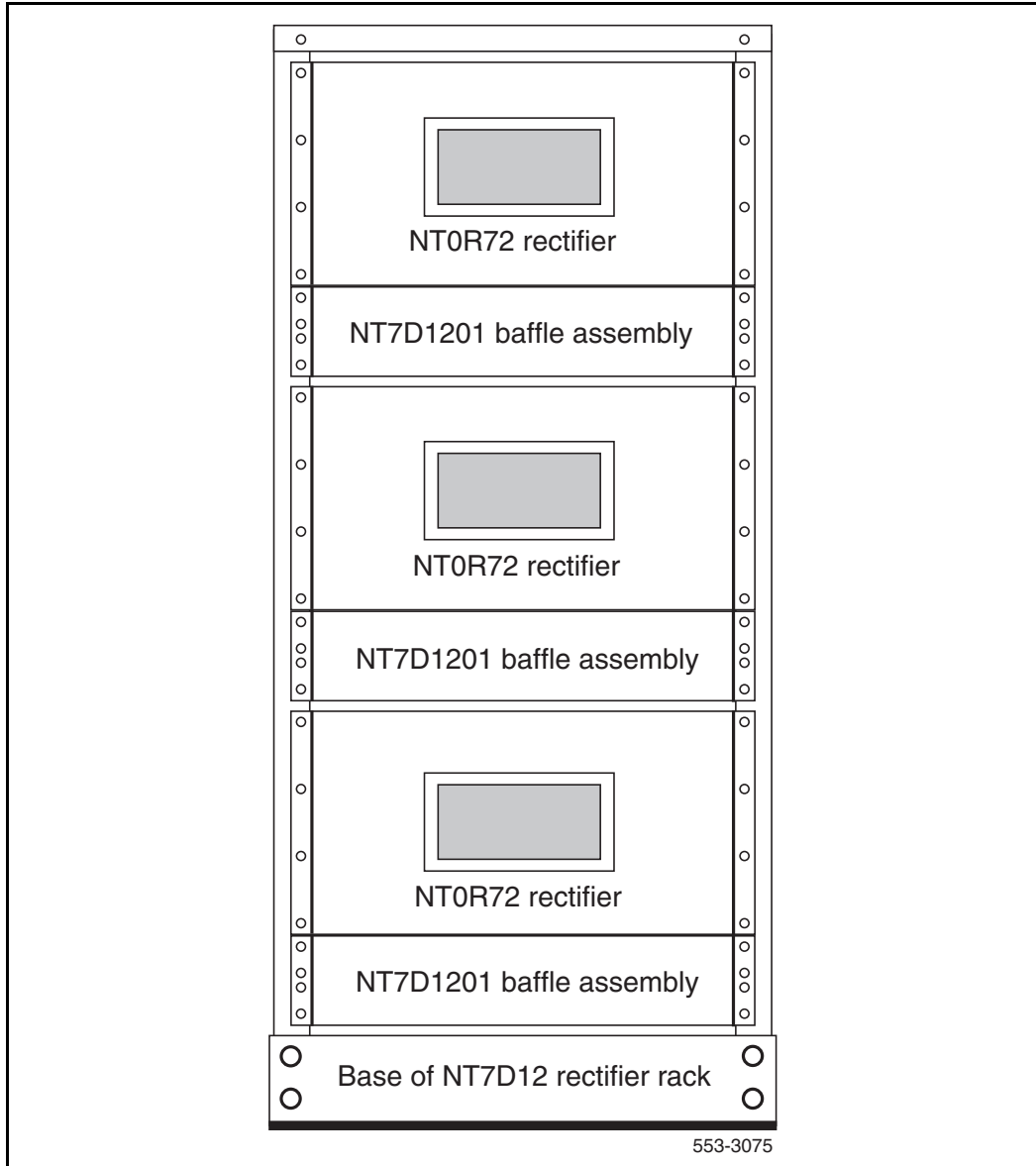
Figure 12 NT7D12 Rectifier Rack Assembly with three NT0R72 rectifiers
