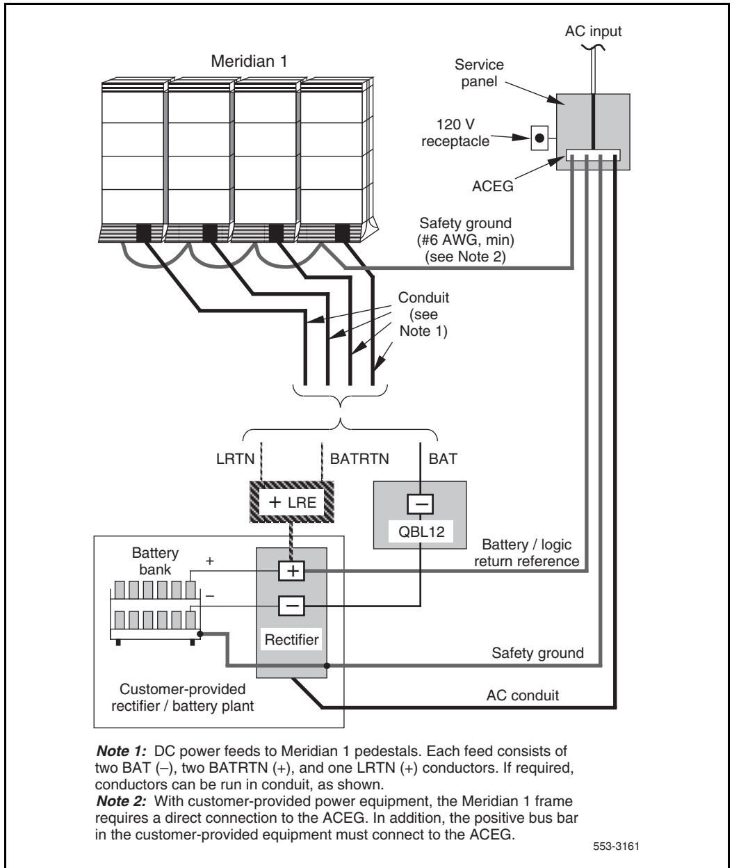
Figure 22 DC power—multiple-column distribution with QBL12 and customer power
