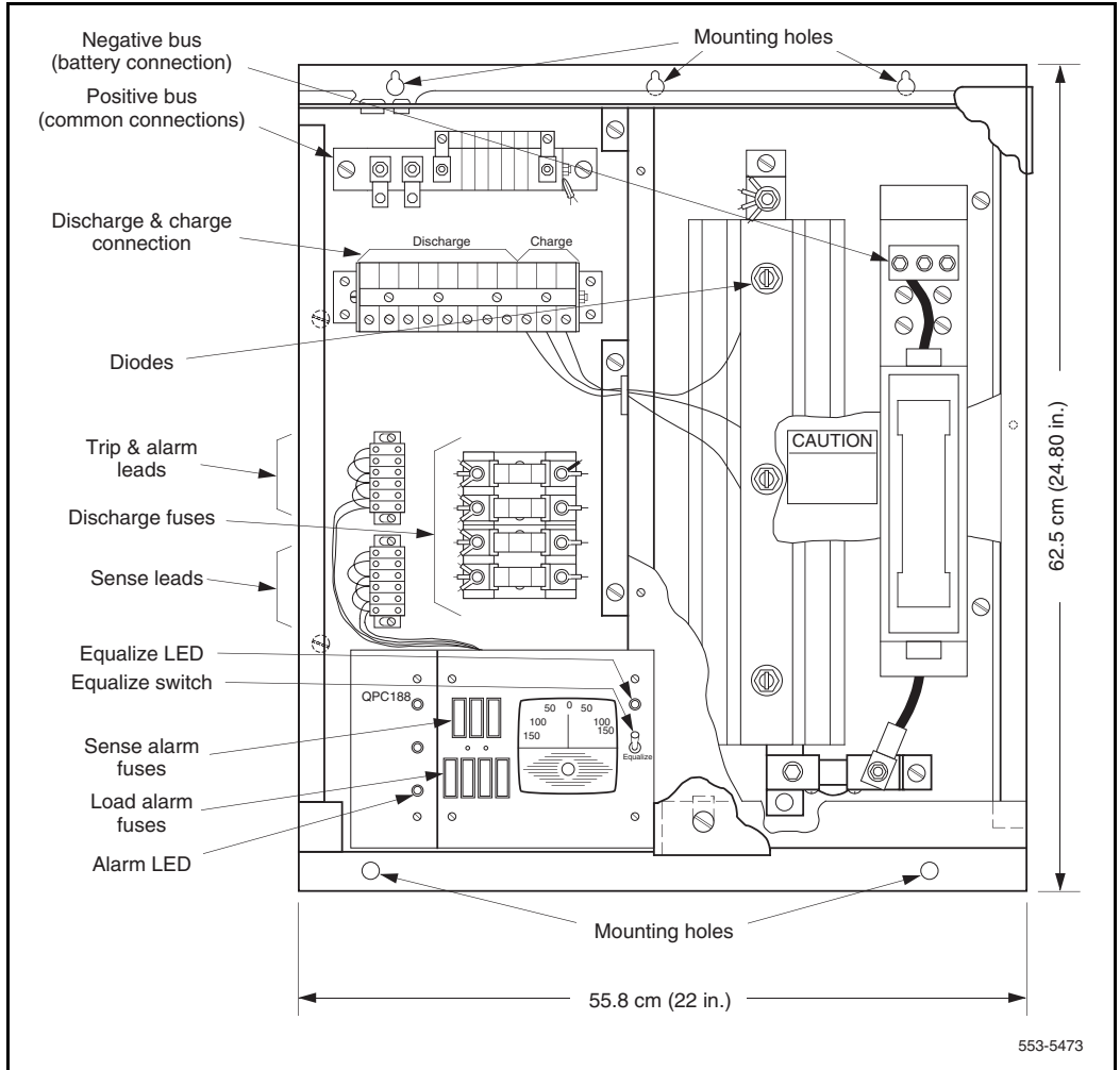
Figure 13 QBL15 Power Distribution Box
