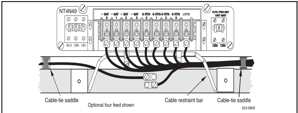
Figure 38 NT4N49 field wiring terminals
