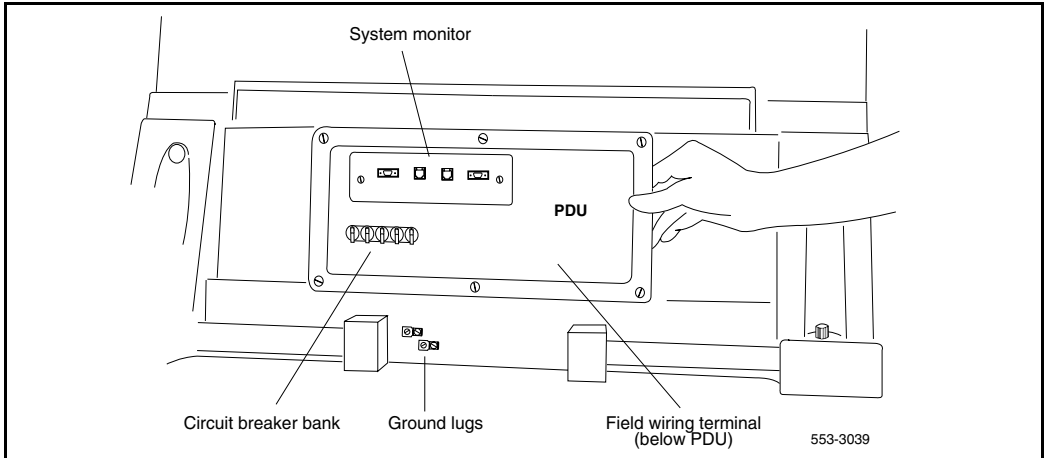
Figure 36 NT4N50 DC PDU
