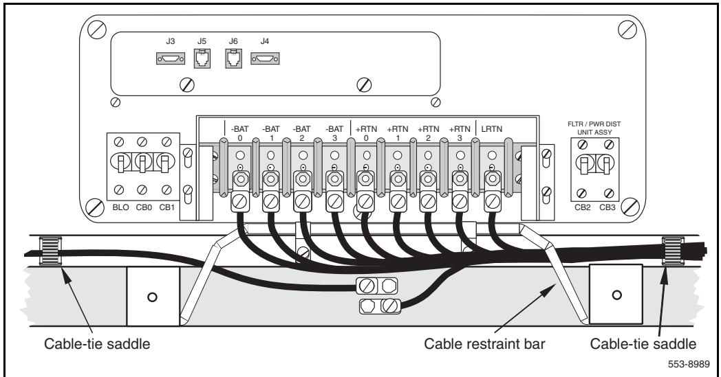
Figure 32 Cable routing in the rear of the pedestal—NT4N49 DC PDU with optional 4 feed wiring
