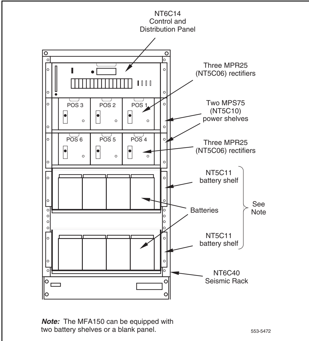
Figure 15 MFA150 Modular Power System with six MPR25 rectifiers
