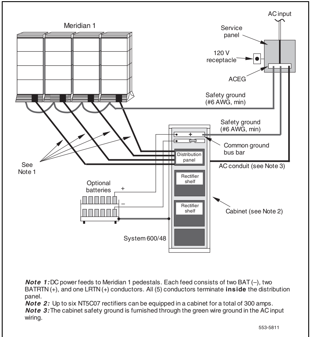
Figure 20 DC power—multiple-column distribution with System 600/48 Power Plant
