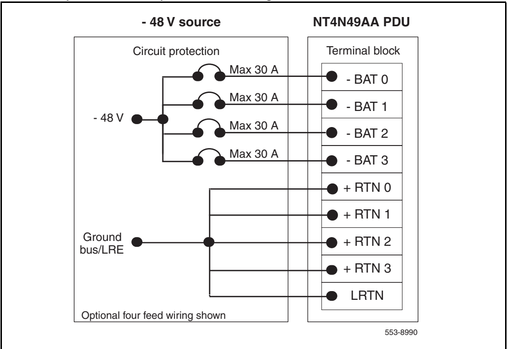
Figure 29 PDU circuit protection with optional 4 feed wiring
