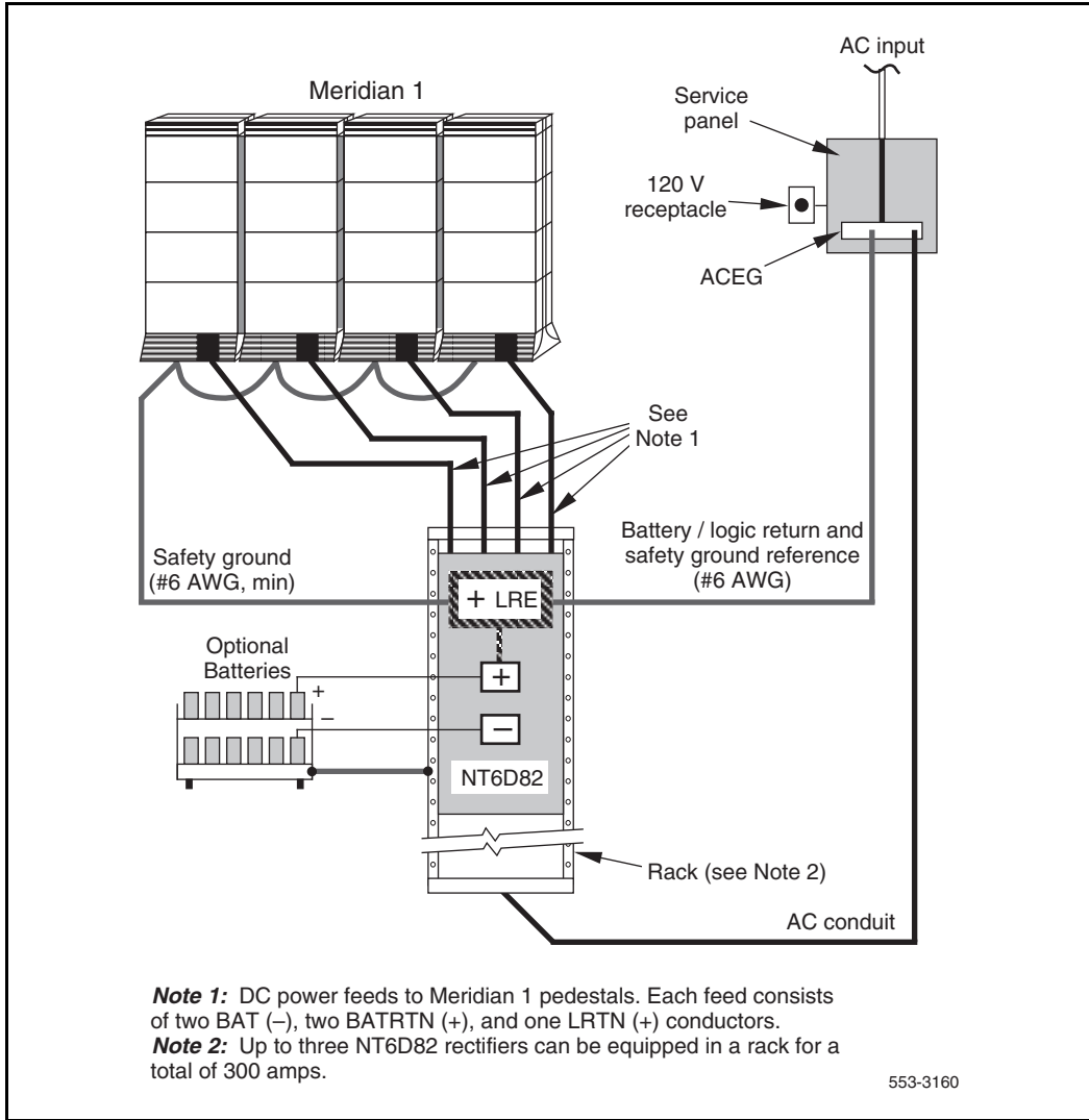
Figure 21 DC power—multiple-column distribution with NT6D82 Power System
