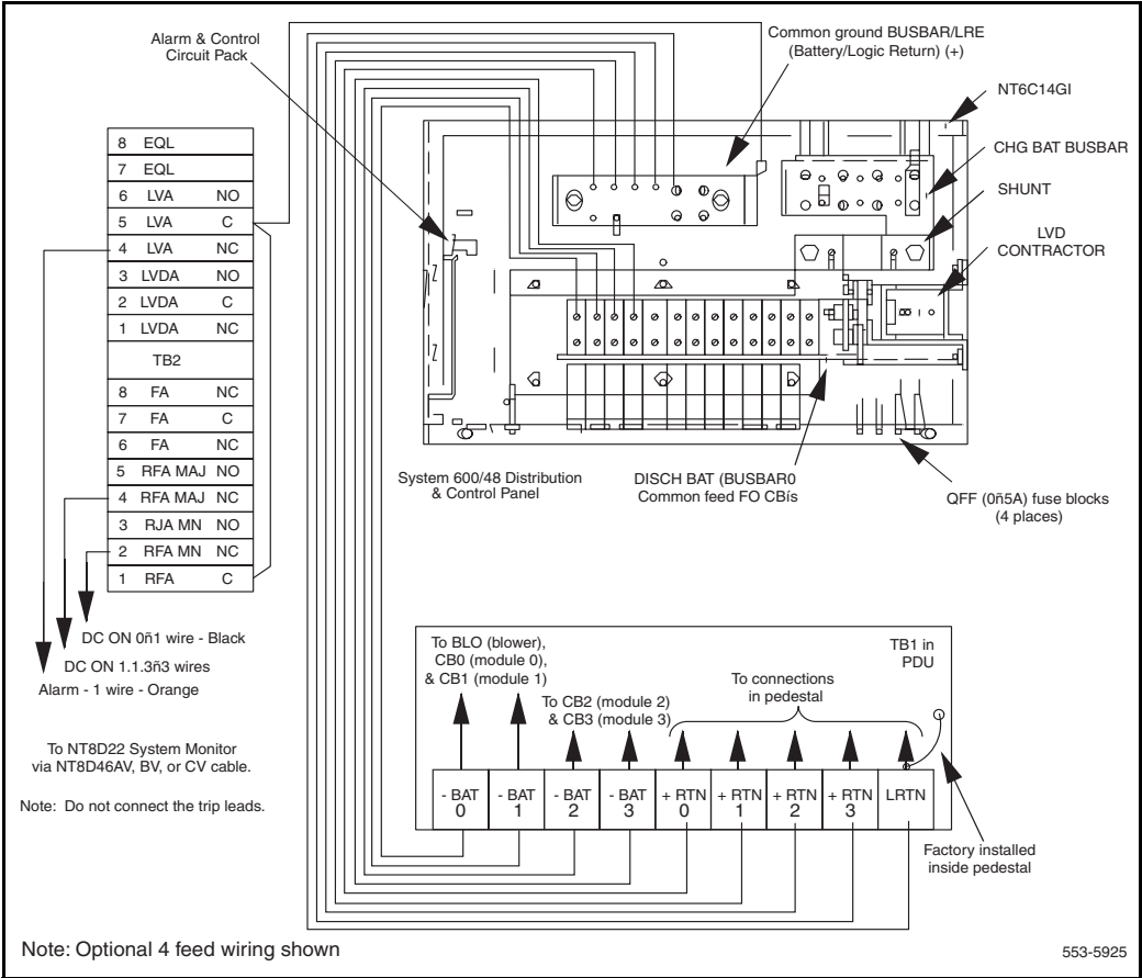
Figure 34 PDU to System 600/48 Power Plant connections
