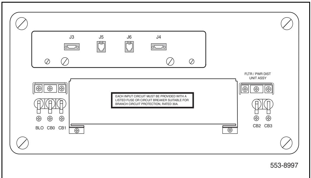
Figure 30 DC power equipment in the rear of the pedestal—NT4N49 DC PDU
