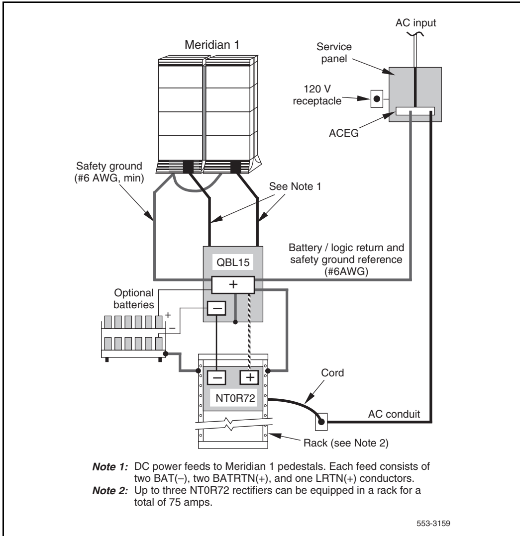
Figure 23 DC power—multiple-column distribution with NT0R72 rectifier and QBL15 Power Distribution Box
