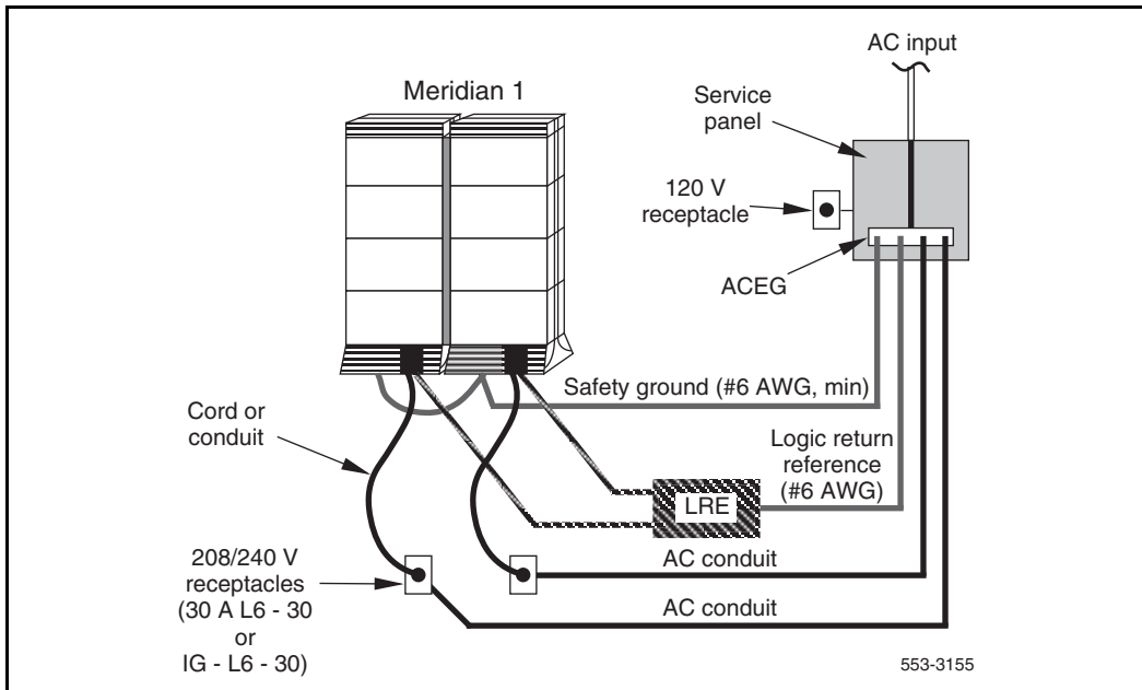
Figure 6 AC power—multiple-column distribution
