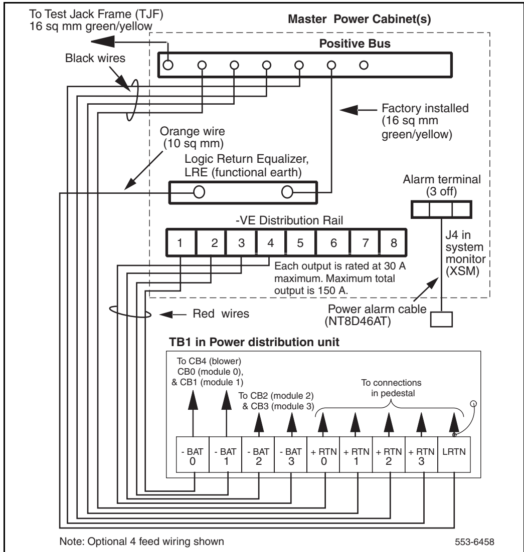
Figure 35 UEM to 8B/4R Master Power Cabinet 2R or 8B/4R Master Power cabinet connections
