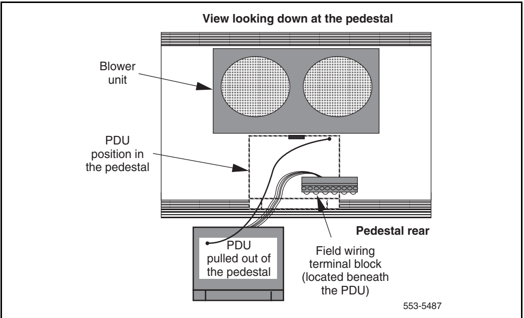
Figure 37 Cabling between the PDU and the field wiring terminal blocks
