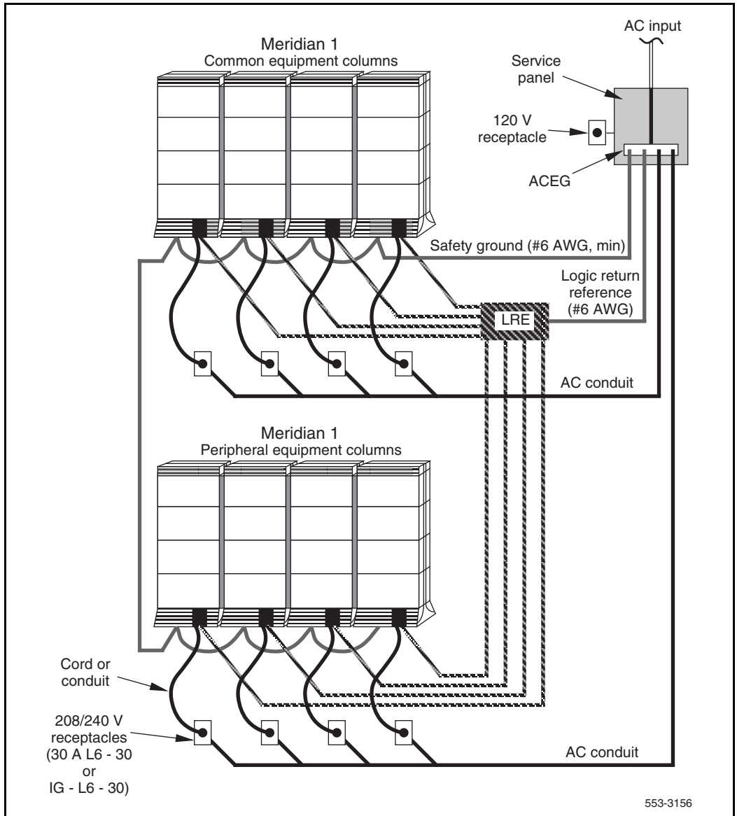
Figure 7 AC power—multiple-row distribution
