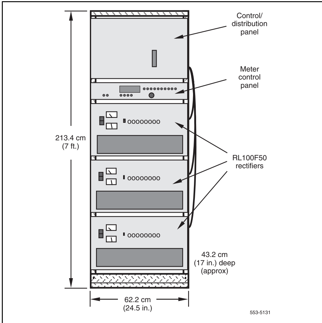
Figure 18 NT6D82 power bay configuration with three RL100F50 rectifiers
