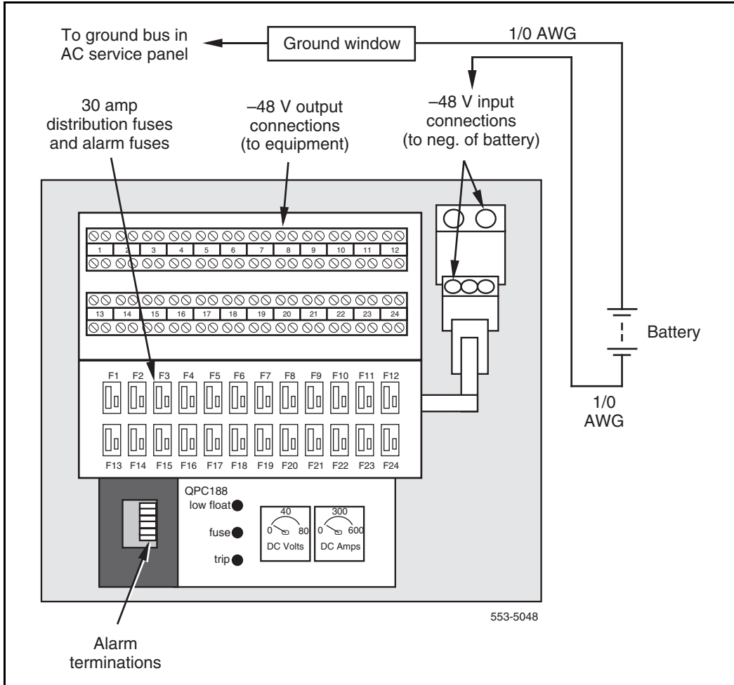
Figure 17 QBL12 Power Distribution Box
