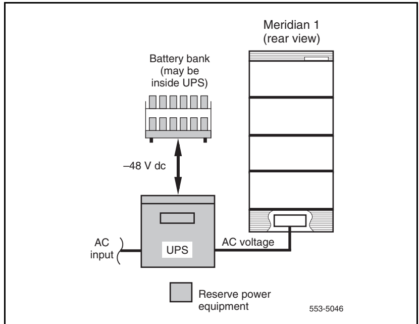
Figure 2 AC-powered system with reserve power
