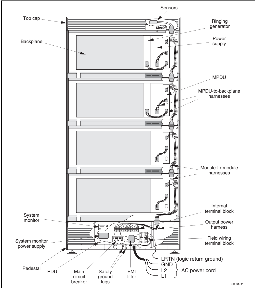
Figure 10 AC internal power distribution (rear of the column)
