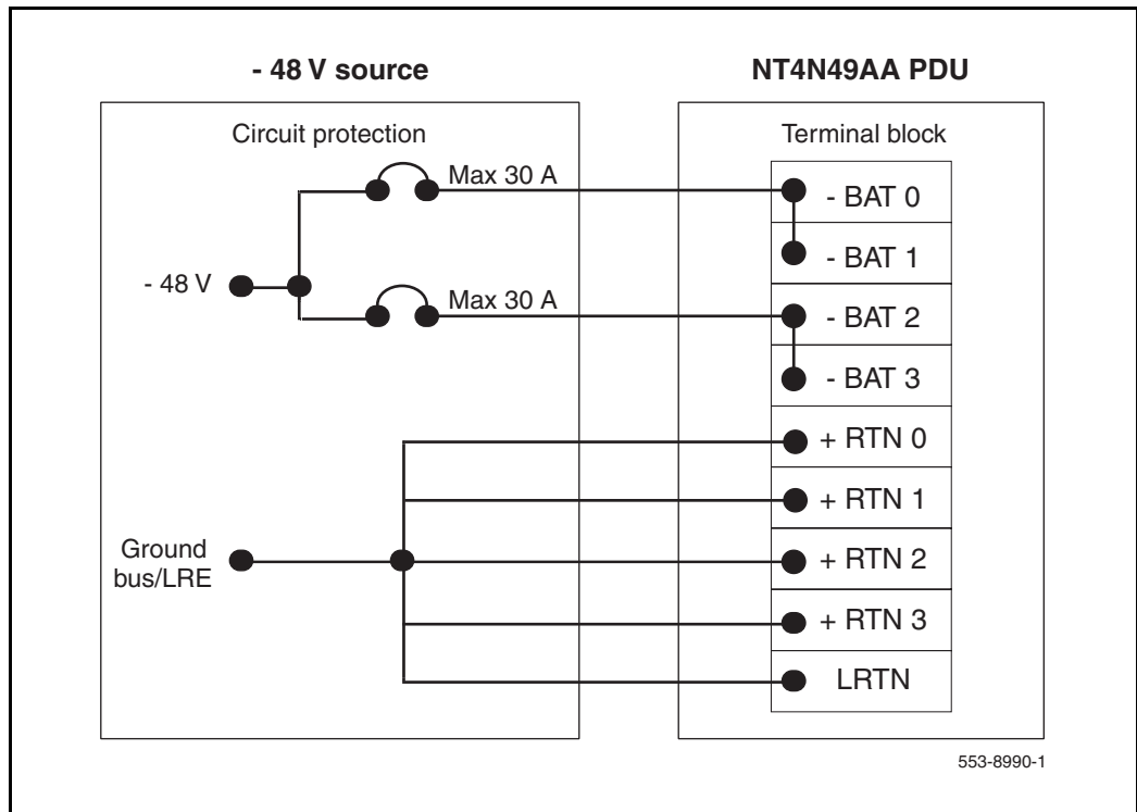
Figure 28 PDU circuit protection with standard 2 feed wiring
