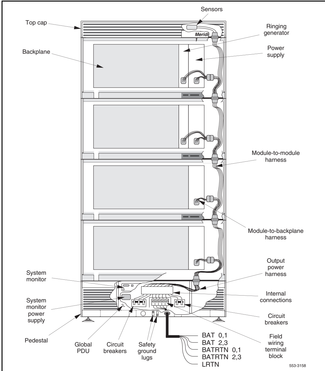
Figure 11 DC internal power distribution (rear of the column)
