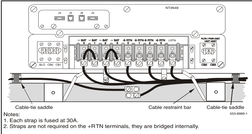
Figure 31 Cable routing in the rear of the pedestal—NT4N49 DC PDU with standard 2 feed wiring
