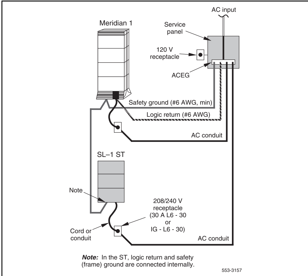
Figure 8 AC power—upgraded system distribution
