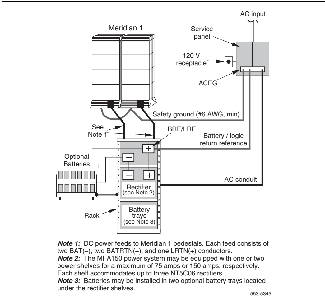
Figure 19 DC power—multiple-column distribution with MFA150 Modular Power System
