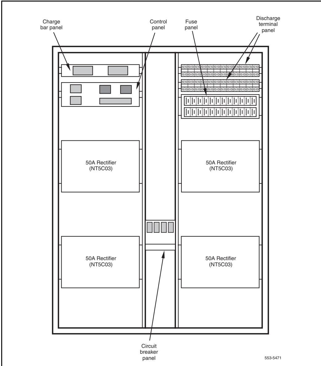
Figure 16 QCA13 Main Power Cabinet Assembly
