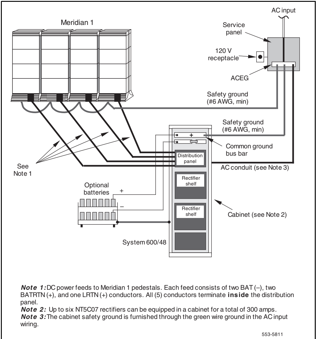
Figure 27 External DC power and ground wiring
