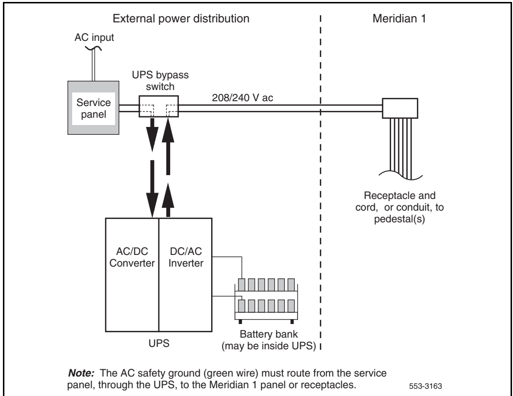
Figure 14 AC reserve power configuration
